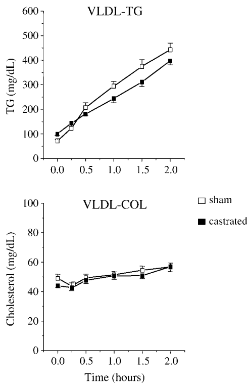
Fig. 1. Hepatic VLDL secretion in castrated and sham-operated cholesteryl ester transfer protein (CETP) transgenic mice measured after Triton WR1339 injection. Values shown are means ± SEM (n = 6–7). Slopes of the triglyceridemia curves are 185.9 ± 12.5 and 144.1 ± 6.0 mg/dl/h for sham-operated and castrated mice, respectively ( P < 0.02). Slopes of cholesterolemia curves are 6.9 ± 0.2 and 7.3 ± 1.7 mg/dl/h for sham-operated and castrated mice, respectively. COL, cholesterol; TG, triglyceride.
