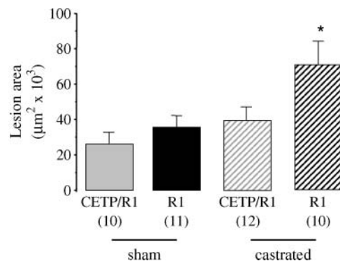
Fig. 4. Areas of aortic lipid-stained lesions in castrated and sham-operated LDL receptor-deficient mice expressing CETP (CETP/R1) or not (R1) after 10 weeks on a high-fat and high-cholesterol diet. Values shown are means \pm SEM ( n ). Statistical comparisons by one-way ANOVA followed by Student-Newman-Keuls test: P = 0.005 . * Castrated R1 mice differ from the other three groups ( P < 0.05 ).
