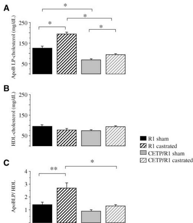
Fig. 3. Cholesterol distribution in plasma lipoprotein fractions from castrated and sham-operated LDL receptor-deficient mice expressing CETP (CETP/R1) or not (R1) after 10 weeks on a high-fat and high-cholesterol diet. A: Apolipoprotein B-containing lipoprotein (apoB-LP)-cholesterol. B: HDL-cholesterol. C: ApoB-LP/HDL ratio. Values shown are means \pm SEM ( n = 5-9 ). Statistical comparisons by Student's t -test: * P < 0.001 , ** P < 0.02 .
