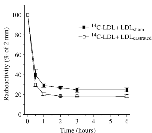
Fig. 2. Competition between LDL from sham-operated (closed symbols) and castrated (open symbols) mice and [ ^{14}\text{C} ]cholesterol-LDL for plasma removal. Labeled LDL from sham-operated mice was mixed with cold LDL from sham-operated or castrated mice and injected into the femoral veins of intact mice (for details, see LDL competition studies in Materials and Methods). Values shown are means ± SD (n = 4). LDL from sham-operated mice more efficiently retarded [ ^{14}\text{C} ]LDL plasma removal than LDL from castrated mice, as shown by the areas under the radioactivity curves (188.9 ± 18.7 vs. 142.1 ± 7.3, sham-operated vs. castrated mice, respectively; P < 0.01 ) and fractional catabolic rates determined from 2 to 60 min (0.020 ± 0.002 vs. 0.027 ± 0.001, sham-operated vs. castrated mice, respectively; P < 0.002 ).
